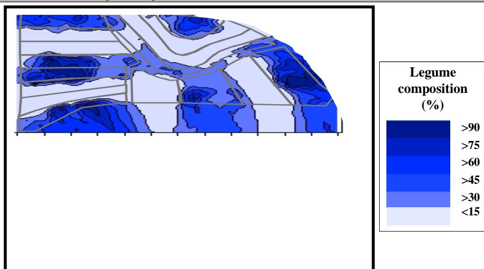
Figure 1. Spatial distribution of mean % legume composition.
