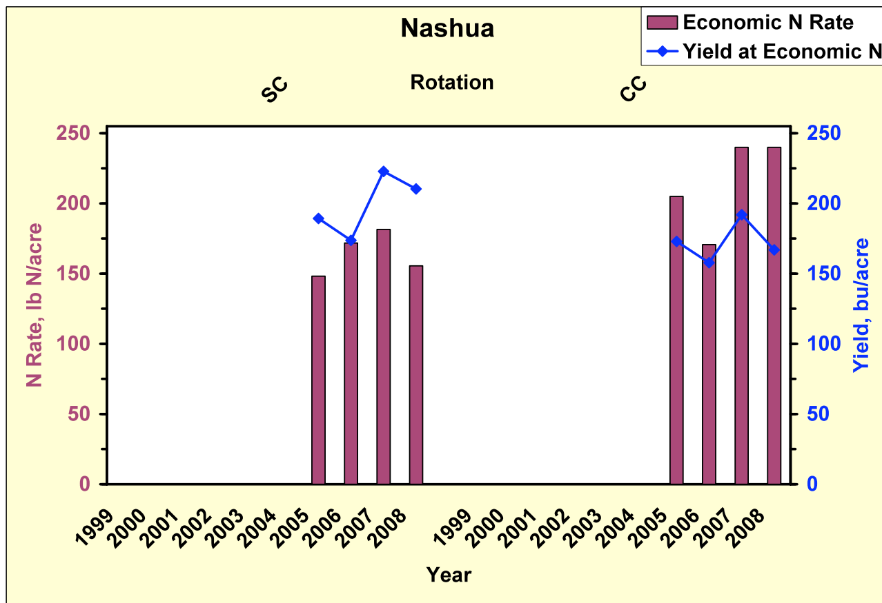
Figure 1. Economic optimum N rate (EONR) and corn yield at the EONR for each rotation and year, Northeast Research Farm, 2005–2008. The EONR was calculated at a 0.10 price ratio ($/lb N:$/bu corn grain).
