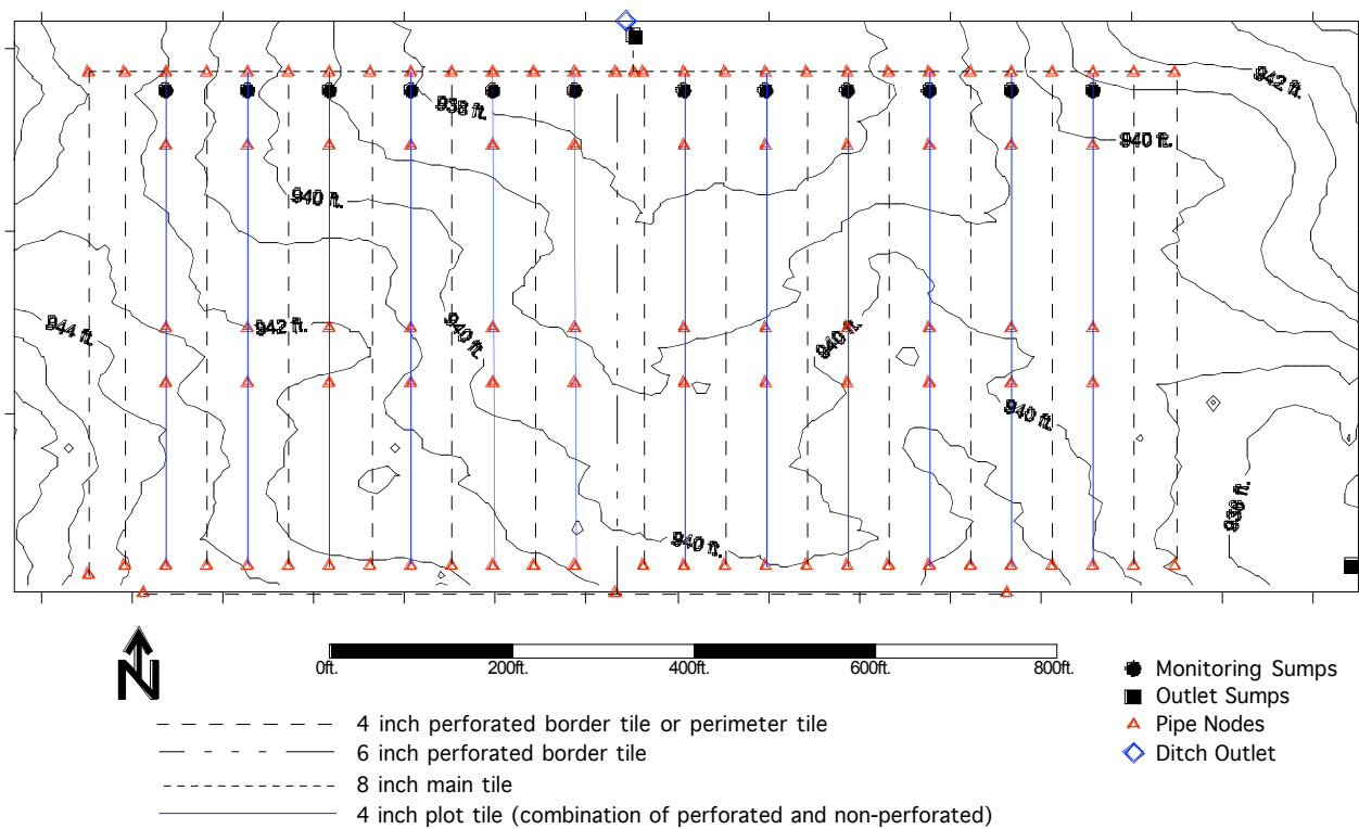
Figure 4. Drainage system layout.
