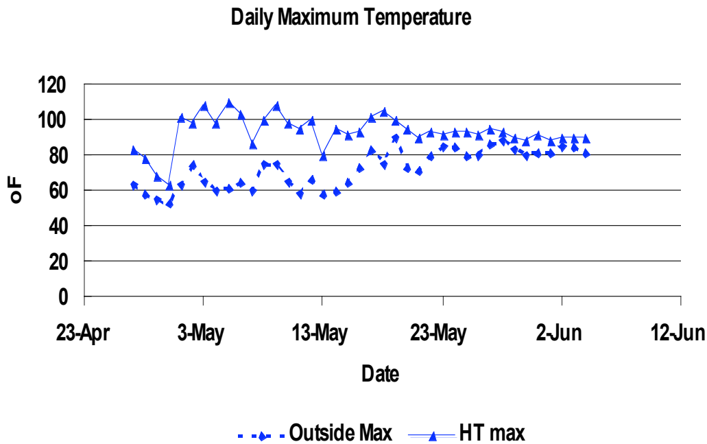
Figure 1. Comparison of outside daily high temperature to high tunnel maximum air temperature. High tunnel temperature probe located between plants at an 8-in. height above the wavelength-selective plastic mulch. Average of three locations. Armstrong Research Farm, Lewis, IA.
