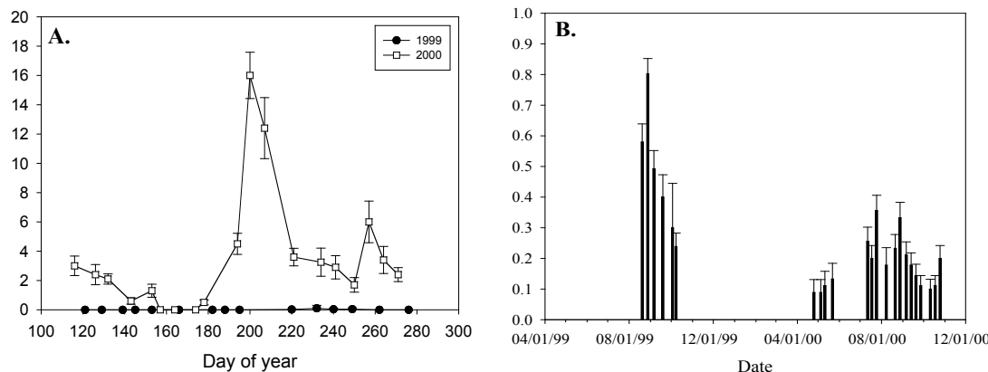
Figure 1. Corn flea beetle population dynamics (A) at the Iowa State University Northeast Research Farm in Nashua, IA, in 1999 and 2000, and (B) the proportion of infested corn flea beetles in 1999 and 2000 (Reference points for (A): DOY 120 = April 30, DOY 180 = June 29, and DOY 240 = August 28).
