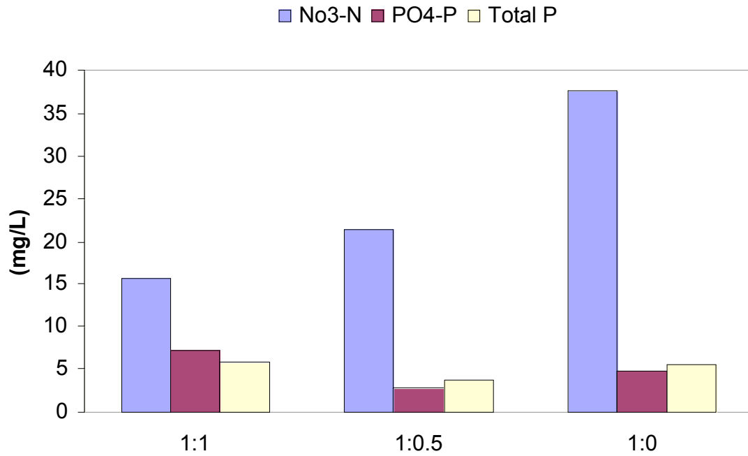
Figure 5. Effect of VFS on average concentration of NO 3 -N, PO 4 -P, and Total P in surface runoff for E1 (June 25, 2003).
