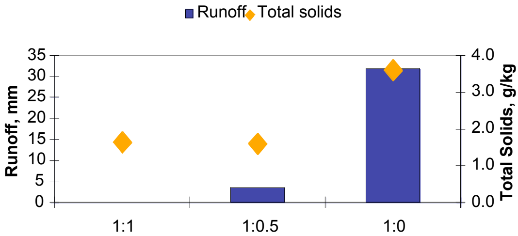
Figure 4. Effect of VFS on average Runoff and Total Solids for E1 (June 25, 2003).
